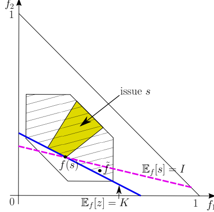
Figure 2: Illustration for Pricing Lemma
