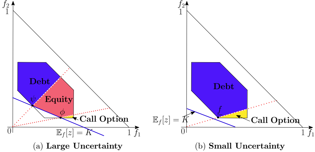
Figure 4: Equilibrium Characterization in the Model with Three States
