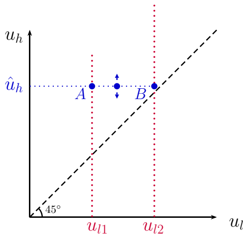
Figure 6: A graphical illustration of why F_l cannot be flat.
