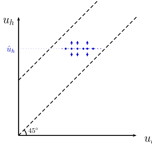
Figure 7: A graphical illustration of why F_h cannot have a mass point.
