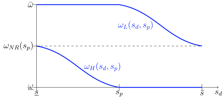
Figure 2: The bank’s investment thresholds \omega_H(s_d, s_p) and \omega_L(s_d, s_p) induced by sending a high message and low message, respectively, as functions of s_d while holding s_p fixed.
